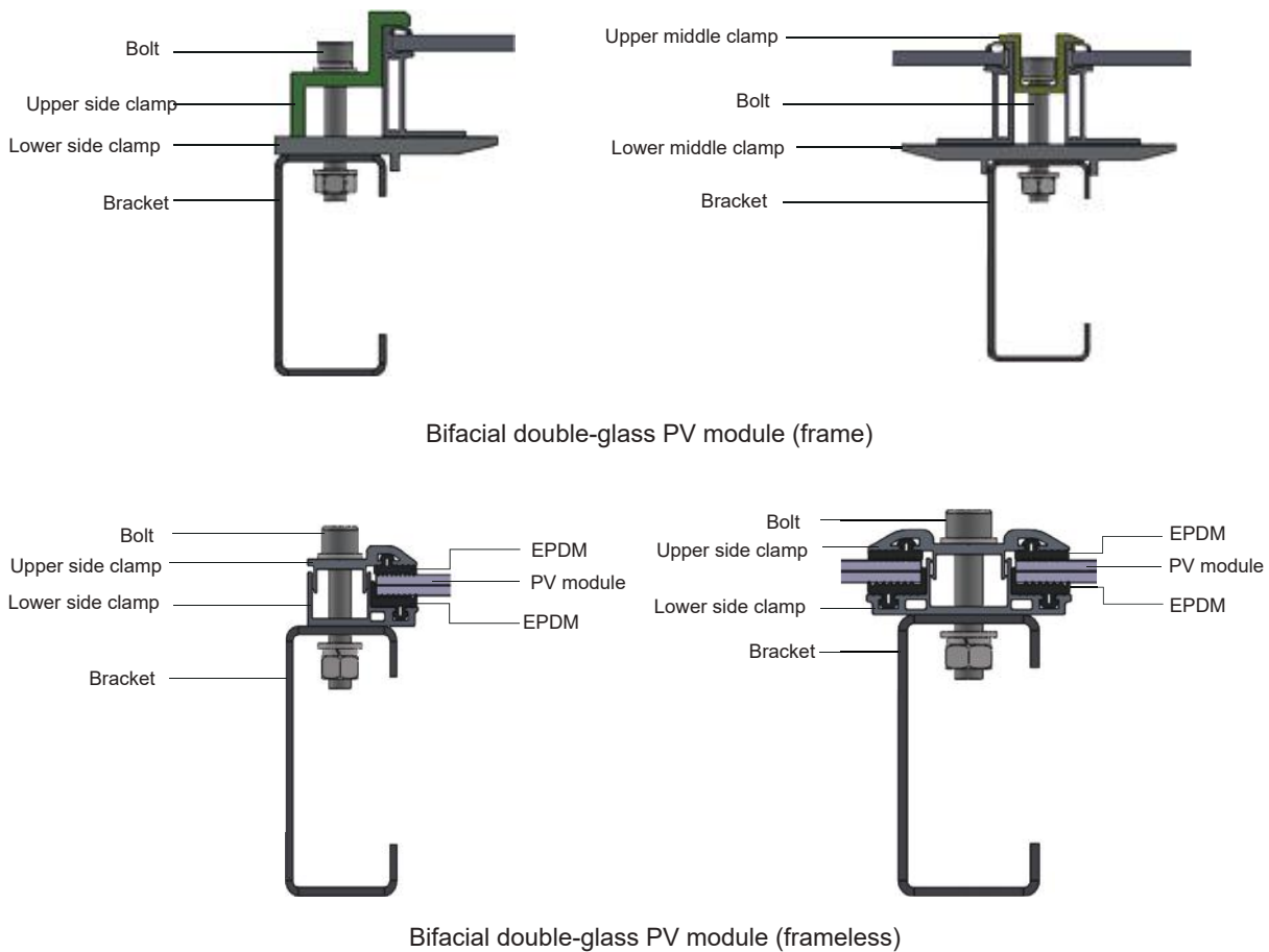
Figure 8 Clamp installation guideline
