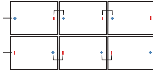
Figure 3 Junction Box Style and Wiring Method
